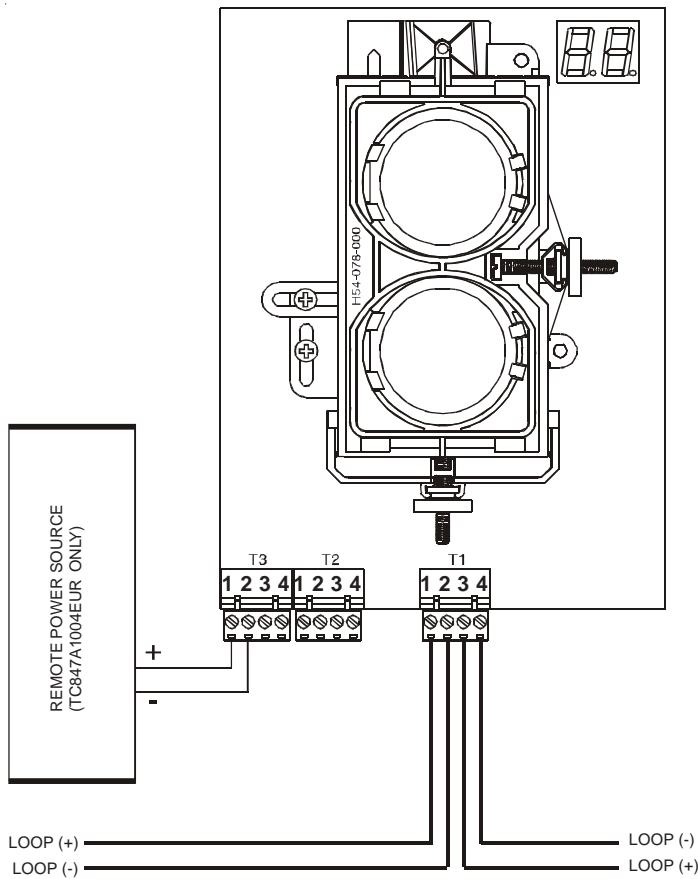
Figure 5: Wiring Diagram
