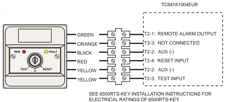
Figure 4: 6500RTS-KEY Wiring
