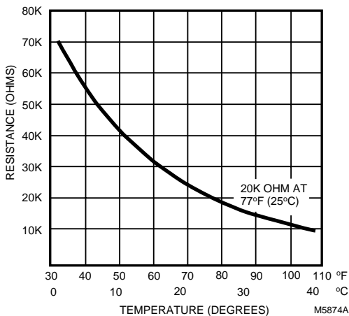
Fig. 1. Temperature vs. resistance for 20k ohm sensor
