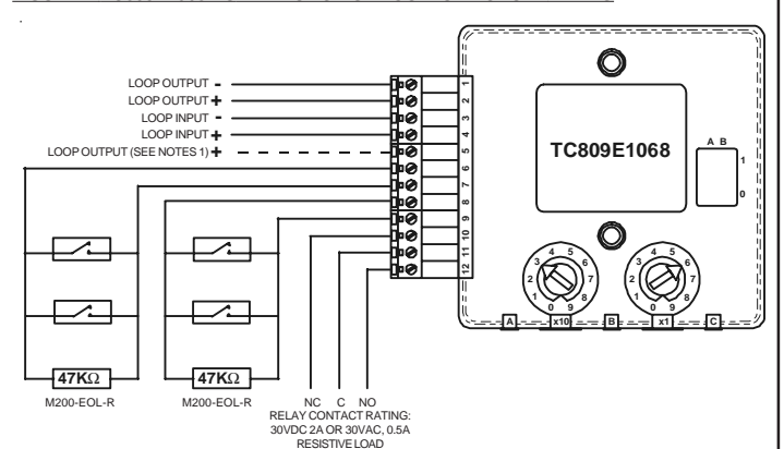
FIGURE 4: TC809E1068 DUAL INPUT SINGLE OUTPUT MODULE WIRING
