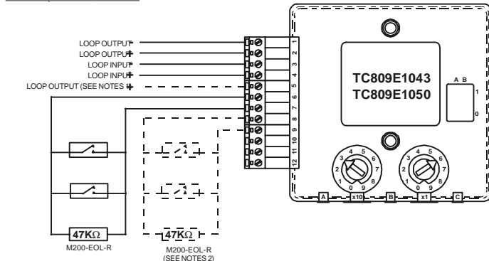
FIGURE 3: TC809E1043 SINGLE INPUT AND TC809E1050 DUAL INPUT MODULE WIRING
