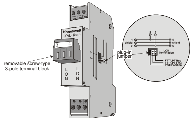
Fig. 9. Lonworks® connection and termination module
