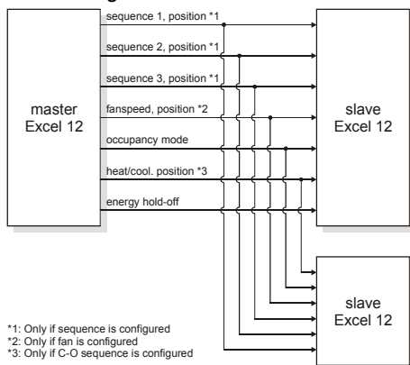
Fig. 3. Master / Slave functionality
