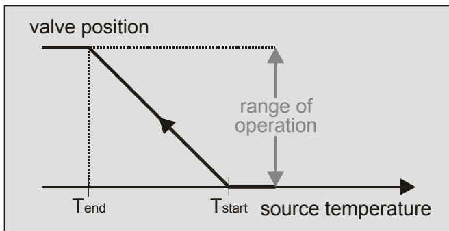
Fig. 2. Minimum Heating Example
